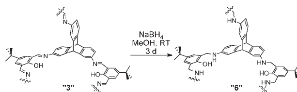
Fig. 4 Reduction of the twelve imine bonds shown exemplified at subunits ("3" and "6") of cage compounds 3 and 6 .
