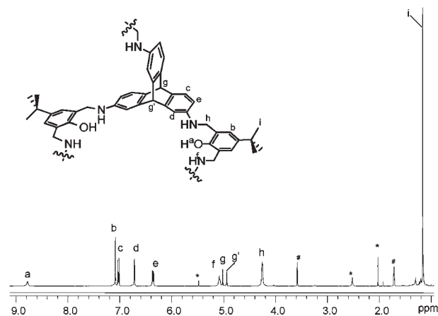
Fig. 5 1 H NMR spectrum of 6 in THF-d 8 (#). The signals labelled with the asterisks (*) are caused by enclathrated solvents (dichloromethane and water).
